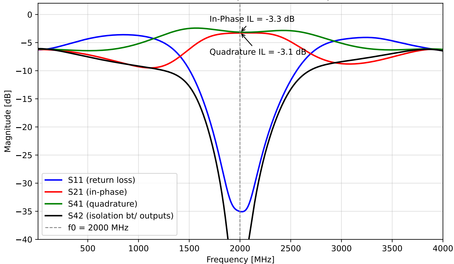
Double-Box Branch-Line Coupler 2000 MHz - S-parameters
