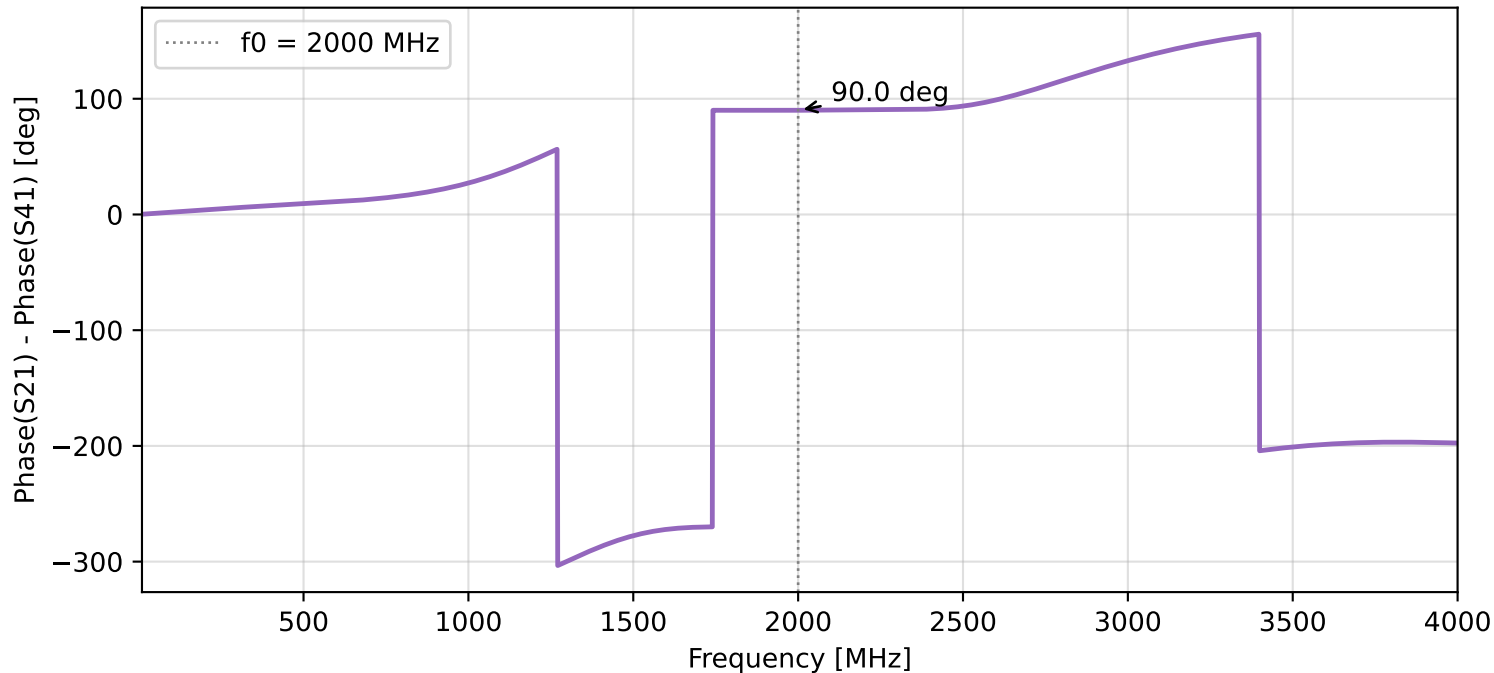
Double-Box Branch-Line Coupler 2000 MHz - Phase difference (I vs Q)
